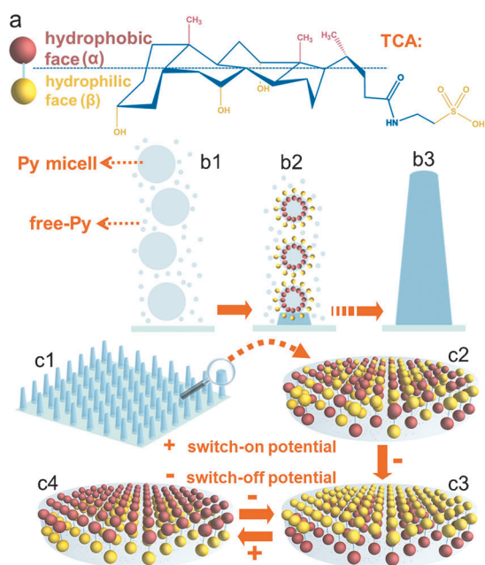
Scheme 1. a) The chair conformation of TCA. b) The possible mechanism of forming 1D NAPPy/TCA ( b3 ) through the self-assembly and polymerization of Py droplets and free-Py (see text for details). c) Proposed mechanism of the electrical-potential-switchable wettability of 1D NAPPy/TCA: c1 – c2 ) The orientation of hydrophobic \alpha -face and hydrophilic \beta -face of TCA was random in the absence of an applied potential. c3 ) The hydrophilic \beta -face of TCA was exposed on the surface of the implants when a switch-off potential was applied to the implants. This state was termed as switch-off. c4 ) When a switch-on potential was applied, the hydrophobic \alpha -face is exposed on the surface, making the implant surface more hydrophobic. This state was termed as switch-on.
